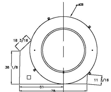
S.S. filter w/ optional Air Flow Optimizer
