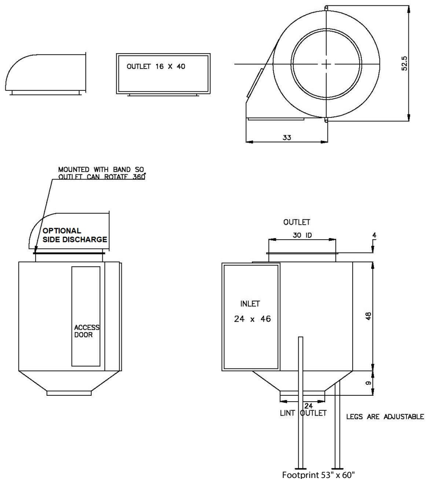
S.S. filter w/ optional Air Flow Optimizer
