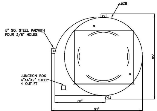
FRP filter w/ optional radius inspection door
