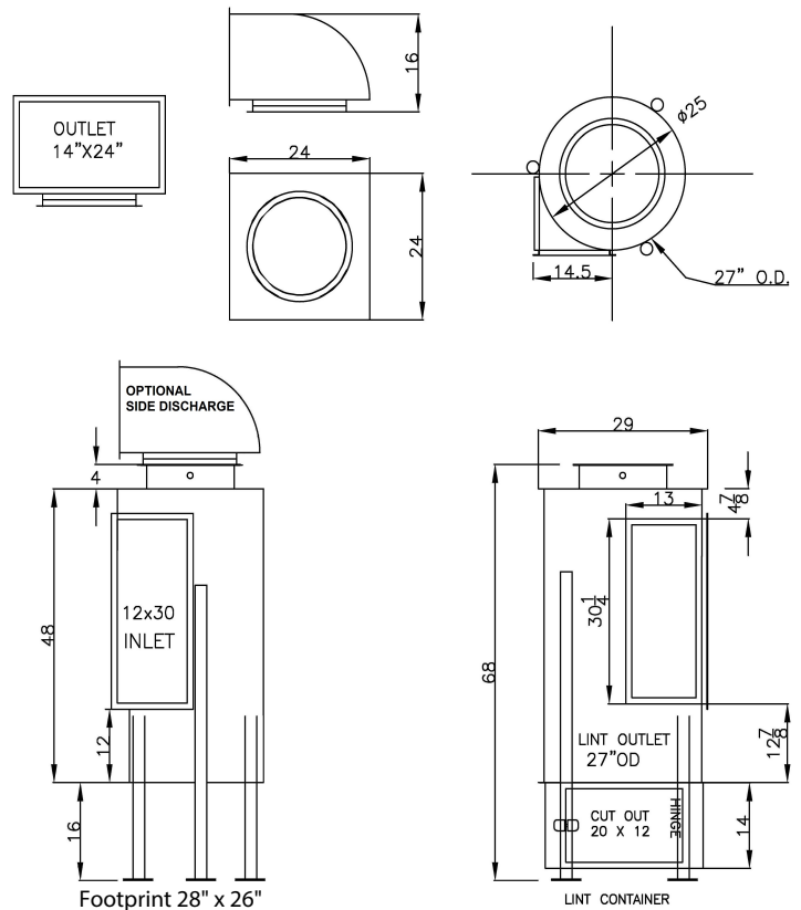
S.S. filter w/ optional Air Flow Optimizer
