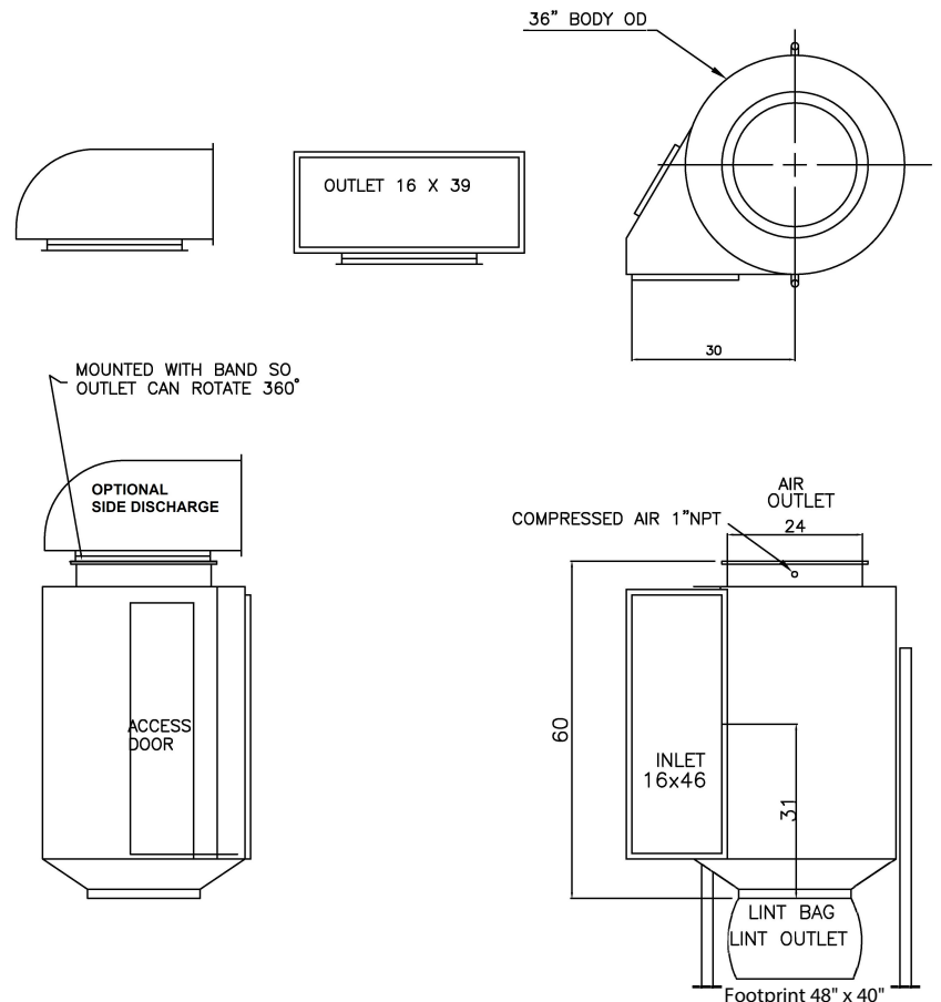
S.S. filter w/ optional Air Flow Optimizer
