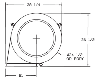
FRP filter w/ optional radius inspection door and compressed air storage tank
