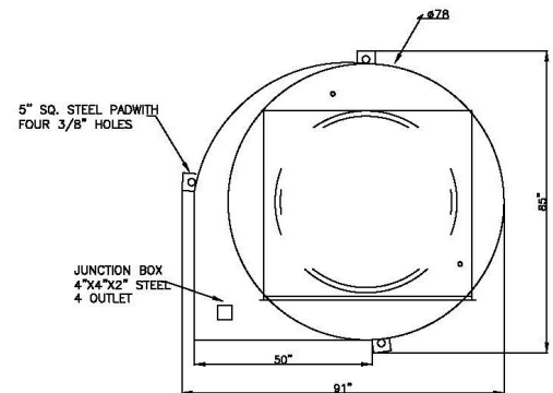
FRP filter w/ optional radius inspection door and compressed air storage tank
