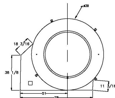
FRP filter w/ optional radius inspection door and compressed air storage tank
