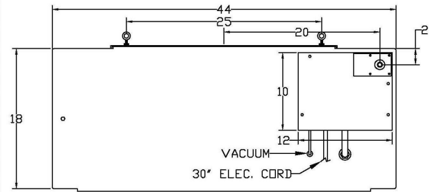
END VIEW
